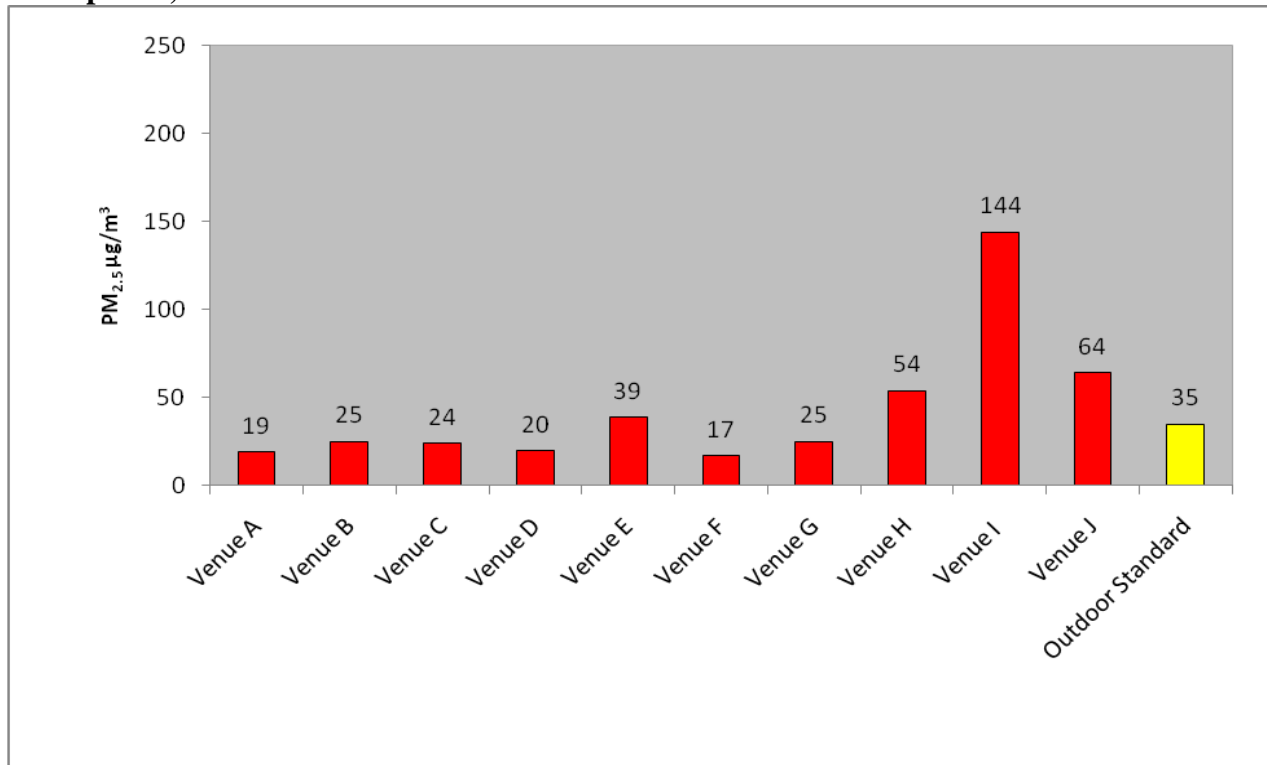
Figure 2. Average Indoor Fine Particle Concentration in 10 Bell County, Kentucky Workplaces, 2011
